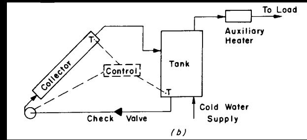
One tank forced circulation system
